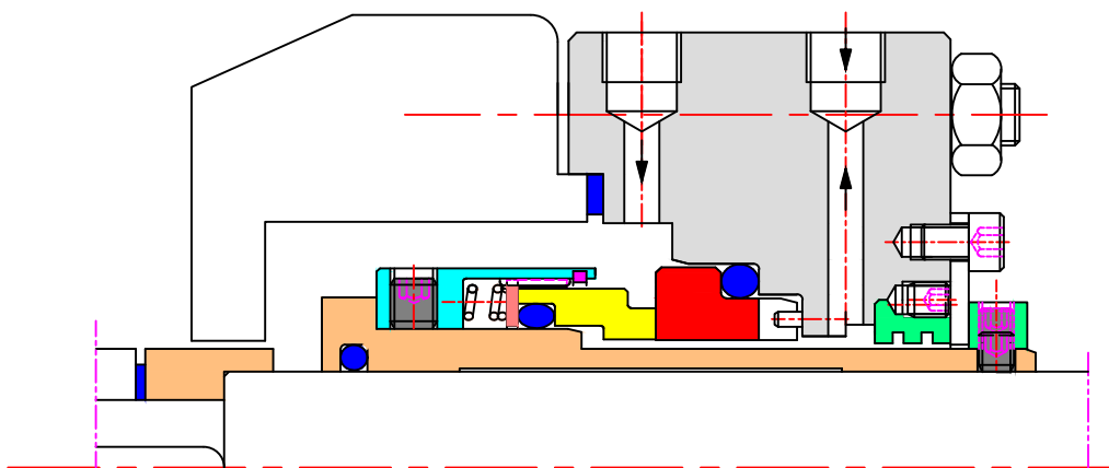
90 SERIES MULTI SPRINGS MECHANICAL SEAL TYPE 9102 CARTRIDGE ARRANGEMENT WITH DIFFERENT API PLAN 11& 62
